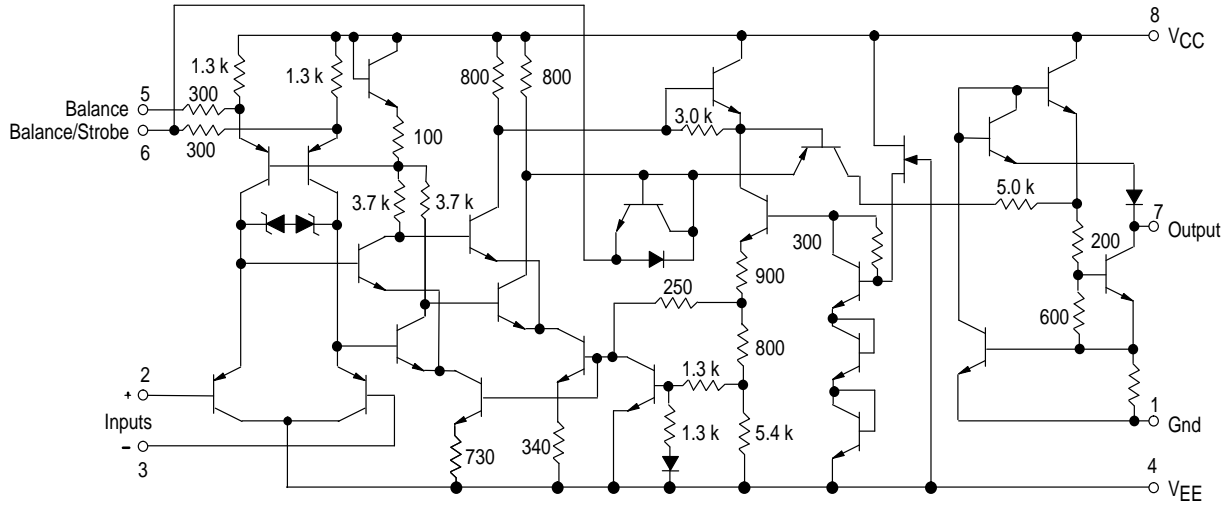
Figure 1. Circuit Schematic
