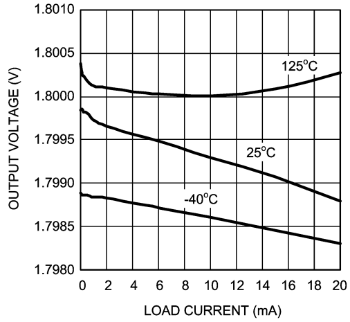
Load Regulation
