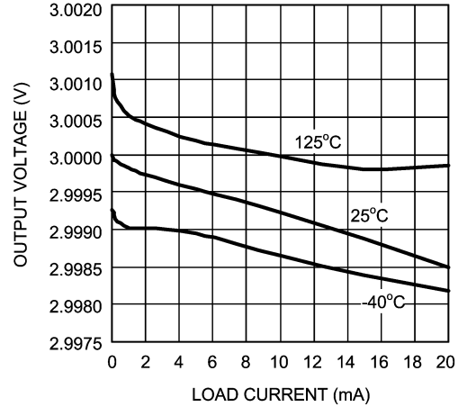
Load Regulation
