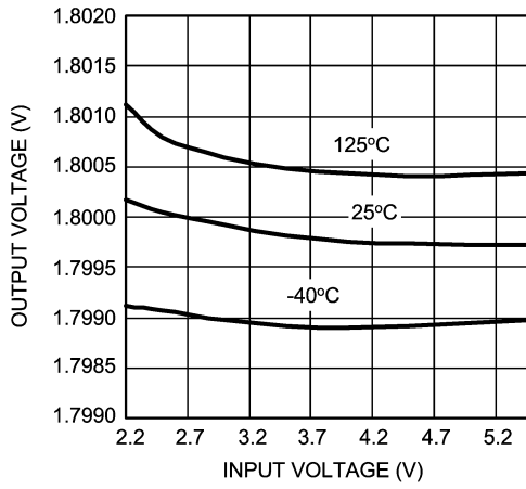
Line Regulation
