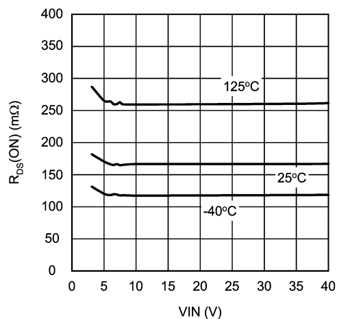
R_{DS(ON)} vs V_{IN} @ I_{SW} = 1A
