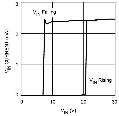
V IN UVLO
