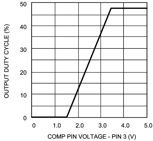
Output Duty Cycle vs Comp Voltage R_T = 16.5k\Omega
