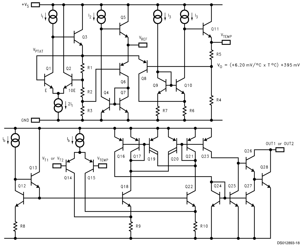
FIGURE 3. Simplified Schematic
