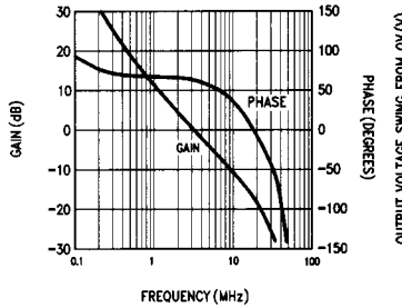
Bode Plot
