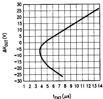
FIGURE 9. t EN2 vs ΔV OUT
