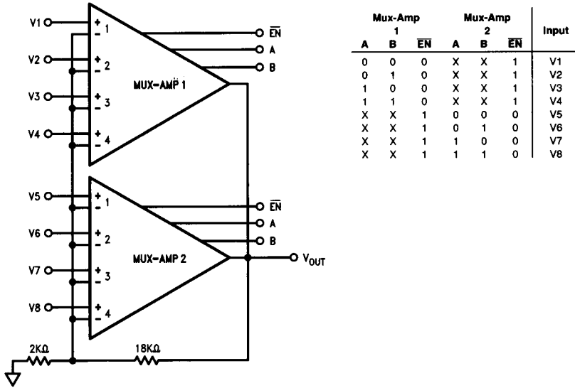
Eight Channel Multiplexer and Amplifier with a Gain of 10
