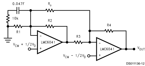
FIGURE 7. Two Op-Amp Instrumentation Amplifier
