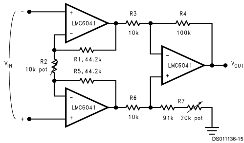
FIGURE 10. Instrumentation Amplifier
