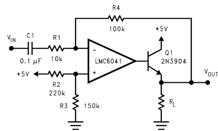
FIGURE 12. AC Coupled Power Amplifier
