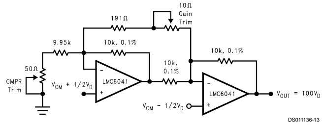
FIGURE 8. Low-Power Two-Op-Amp Instrumentation Amplifier
