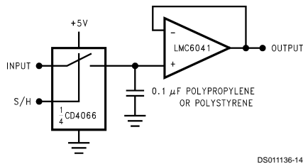
FIGURE 9. Low-Leakage Sample and Hold
