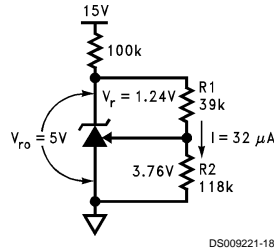
FIGURE 4. Thevenin Equivalent of Reference with 5V Output
