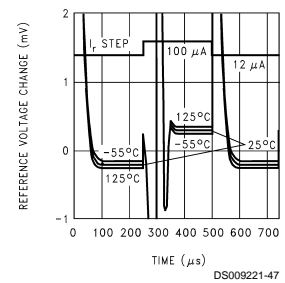
Reference Voltage with 100 ~ 12 uA Current Step
