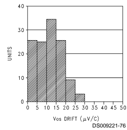
Average V_{OS} Drift Commercial Temperature Range
