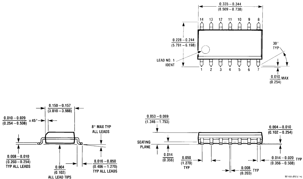
Plastic Surface Mount Narrow Package (0.15) (M) Order Number LM611CM or LM611IM NS Package Number M14A
