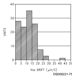
Average V_{OS} Drift Industrial Temperature Range
