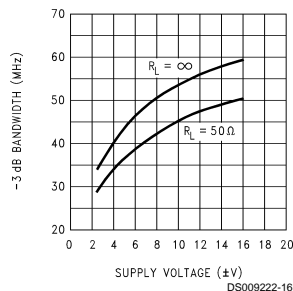
-3 dB Bandwidth
