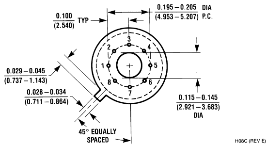
Metal Can Package (H) Order Number LM6125H/883 or LM6125H NS Package Number H08C
