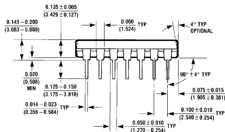
Molded Dual-In-Line Package (N) Order Number LM6225N or LM6325N NS Package Number N14A
