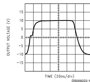
Large Signal Response (RL = 50Ω)
