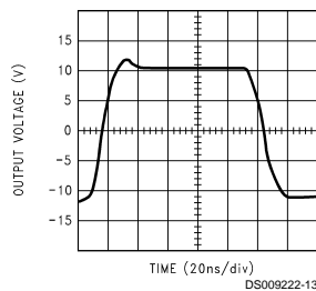
Large Signal Response (RL = 1 kΩ)
