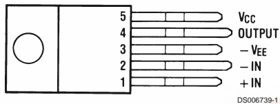
TO-220 Power Package (T)
