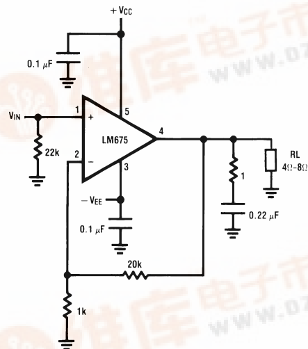
Non-Inverting Amplifier
