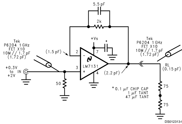
FIGURE 1. Cable Driver A_v = +1
