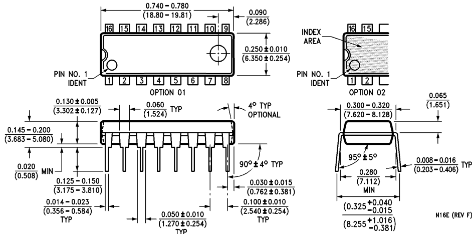
Molded Dual-in-Line Package (N) Order Number LM903N NS Package N16E
