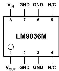
Top View LM9036M-3.3, LM9036M-5.0 See NS Package Number M08A
