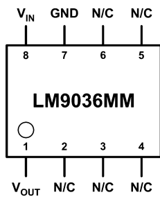
Top View LM9036MM-3.3, LM9036MM-5.0 See NS Package Number MUA08A
