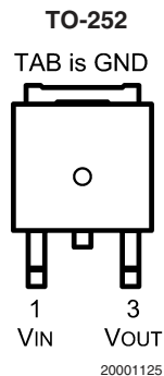
Top View Order Number LM9036DT-5.0, LM9036DT-3.3 See NS Package Number TD03B
