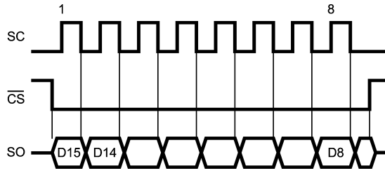
a) Reading Continuous Conversion - Single Eight-Bit Frame
