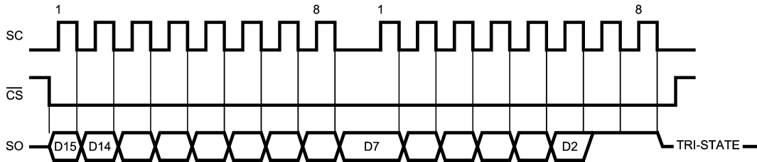
b) Reading Continuous Conversion - Two Eight-Bit Frames
