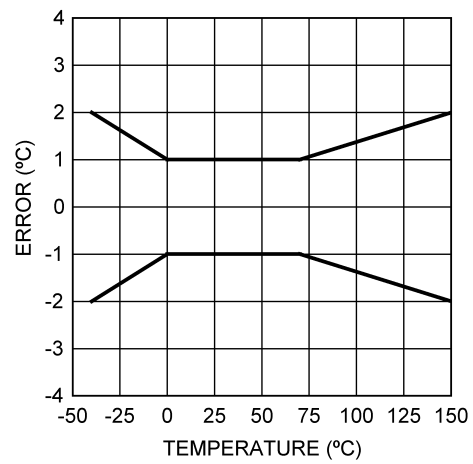
Maximum Temperature Error
