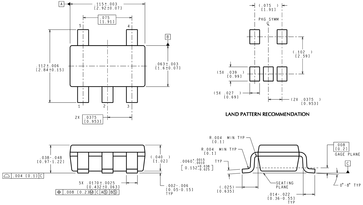
LM95071 Top View SOT23-5 Package NS Package Number MF05A
