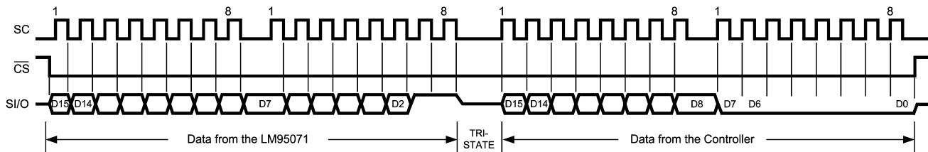
d) Writing Conversion Mode
