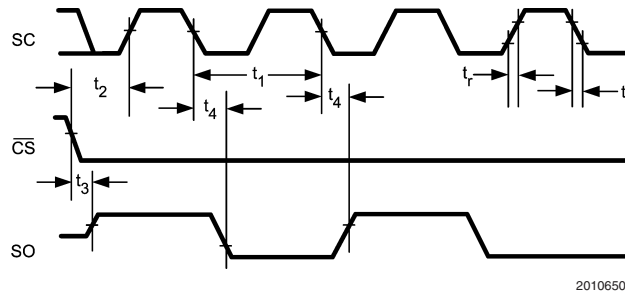
FIGURE 2. Data Output Timing Diagram
