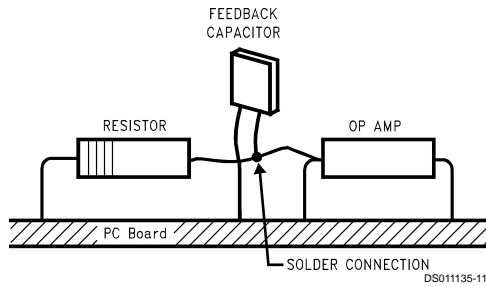
FIGURE 7. Air Wiring
