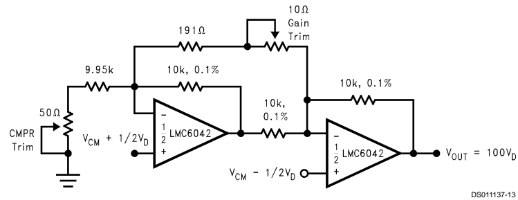
FIGURE 8. Low-Power Two-Op-Amp Instrumentation Amplifier
