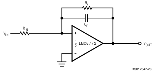
FIGURE 3. Canceling the Effect of Input Capacitance
