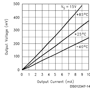
Output Voltage vs Output Current (Sinking) V_S = 15V
