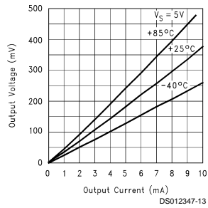
Output Voltage vs Output Current (Sinking) V_S = 5V
