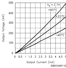
Output Voltage vs Output Current (Sinking) V_S = 2.7V
