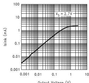
Sinking Output vs Output Voltage
