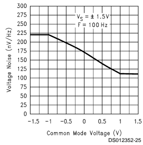
Voltage Noise vs Common Mode Voltage @ 3V
