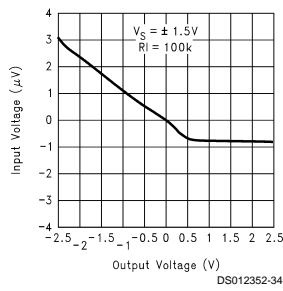
Output Voltage vs Input Voltage @ 5V
