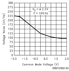
Voltage Noise vs Common Mode Voltage @ 5V
