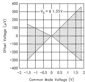
Offset Voltage vs Common Mode Voltage @ 2.7V
