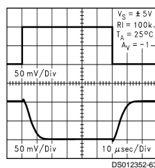
Inverting Small Signal Pulse Response at 10V
