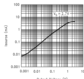
Sourcing Output vs Output Voltage
