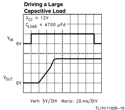
FIGURE 7. Driving a Large Capacitive Load
