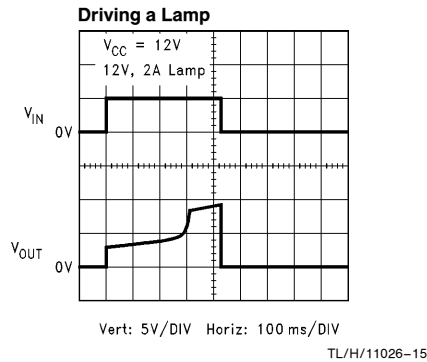
FIGURE 6. Soft Turn-On of a Lamp Load
