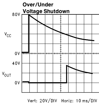
FIGURE 3. Overvoltage/Undervoltage Shutdown
