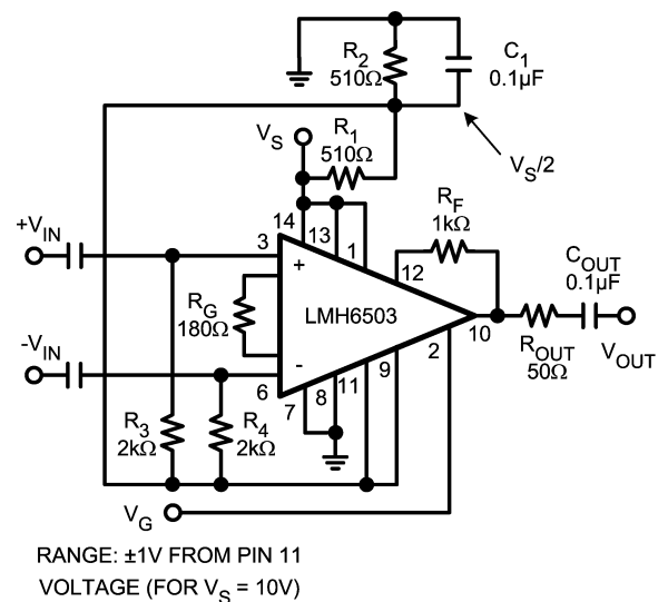
FIGURE 7. AC Coupled Single Supply VOA
