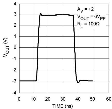
Step Response, 6V_{PP}
