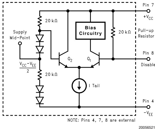
FIGURE 4. Enable/Disable Operation
