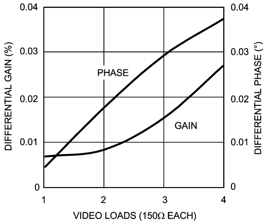
DG/DP (LMH6722)
