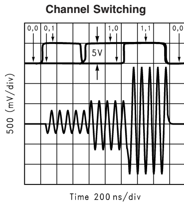
FIGURE 7. PGA Output
