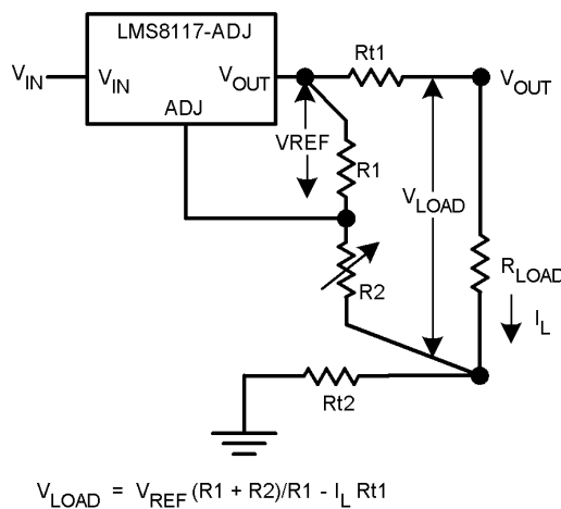
FIGURE 3. Best Load Regulation using Adjustable Output Regulator
