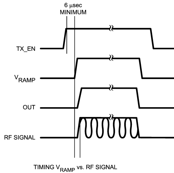
FIGURE 5. Timing V_{\text{RAMP}} vs. RF Signal
