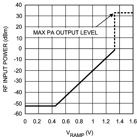
FIGURE 2. P_{\text{IN}} vs. V_{\text{RAMP}}
