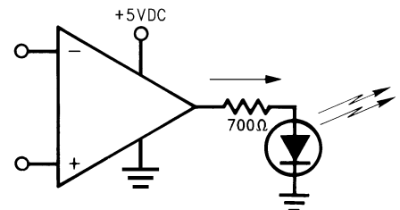
FIGURE 23. LED Driver
