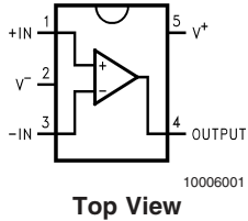
5-Pin SC70-5/SOT23-5
