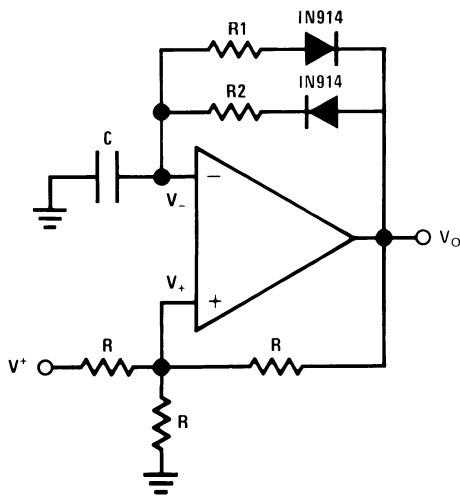
FIGURE 16. Pulse Generator
