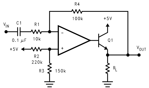
FIGURE 22. Power Amplifier
