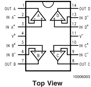
14-Pin SO/TSSOP
