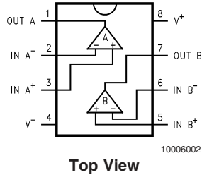
8-Pin SO/MSOP
