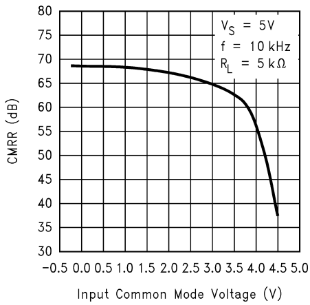
CMRR vs. Input Common Mode Voltage
