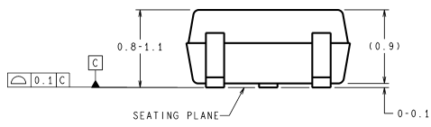
5-Pin SC70-5 NS Package Number MAA05A
