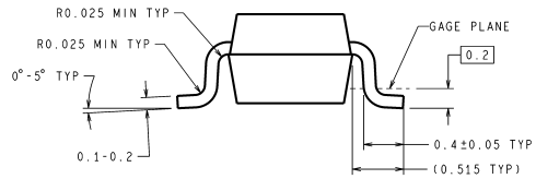
5-Pin SC70-5 NS Package Number MAA05A
