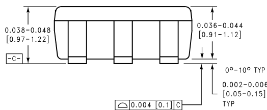
5-Pin SOT23-5 NS Package Number MA05B
