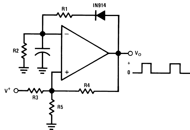
FIGURE 18. Pulse Generator
