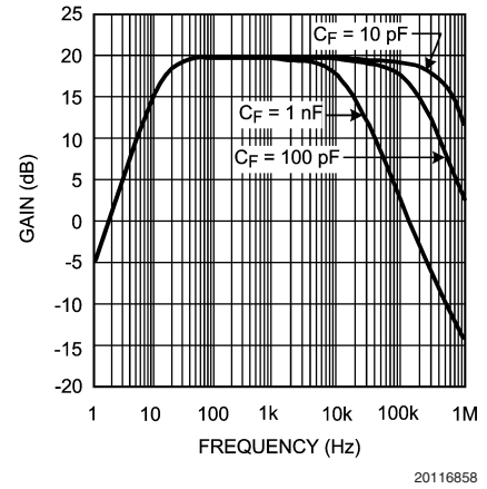
FIGURE 7. Frequency Response of the Inverting Audio Preamplifier
