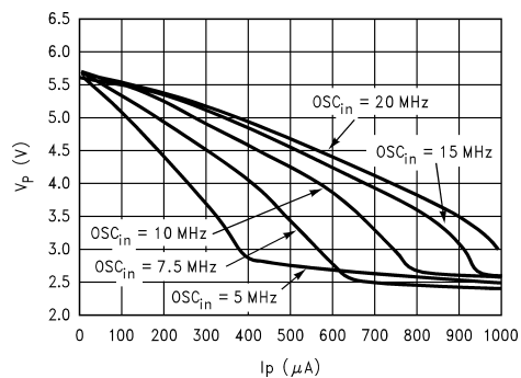
LMX2350 V_p Voltage vs V_p Load Current in Vdoubler Mode, T = 25^\circ C
