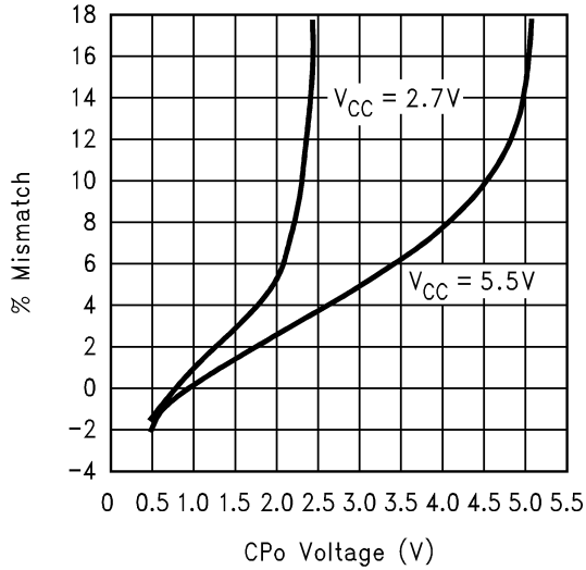
Sink vs Source Mismatch (See (Note 6) under Charge Pump Current Specification Definitions)
