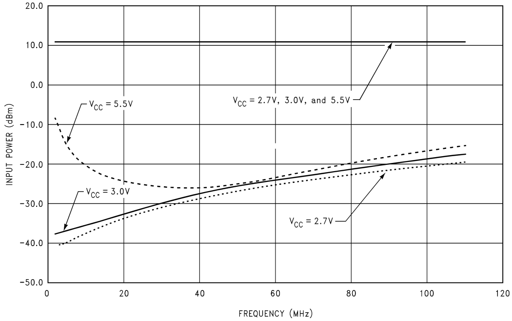
OSCinRF Counter Sensitivity T_A = 25^\circ\text{C}
