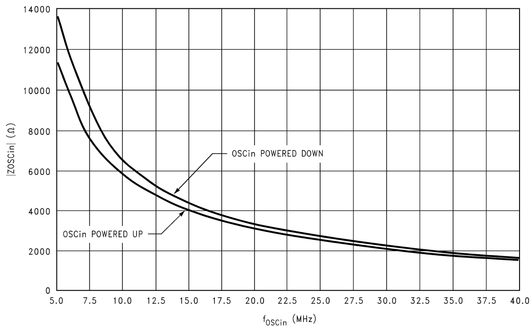
LMX243x UTCSP OSCin Input Impedance Vs Frequency V_{CC} = EN = 2.50V T_A = +25^\circ C
