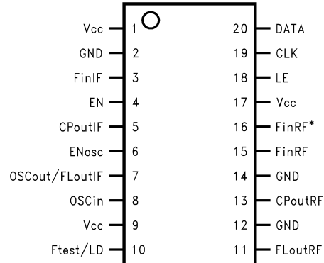
Thin Shrink Small Outline Package (TM) (Top View)
