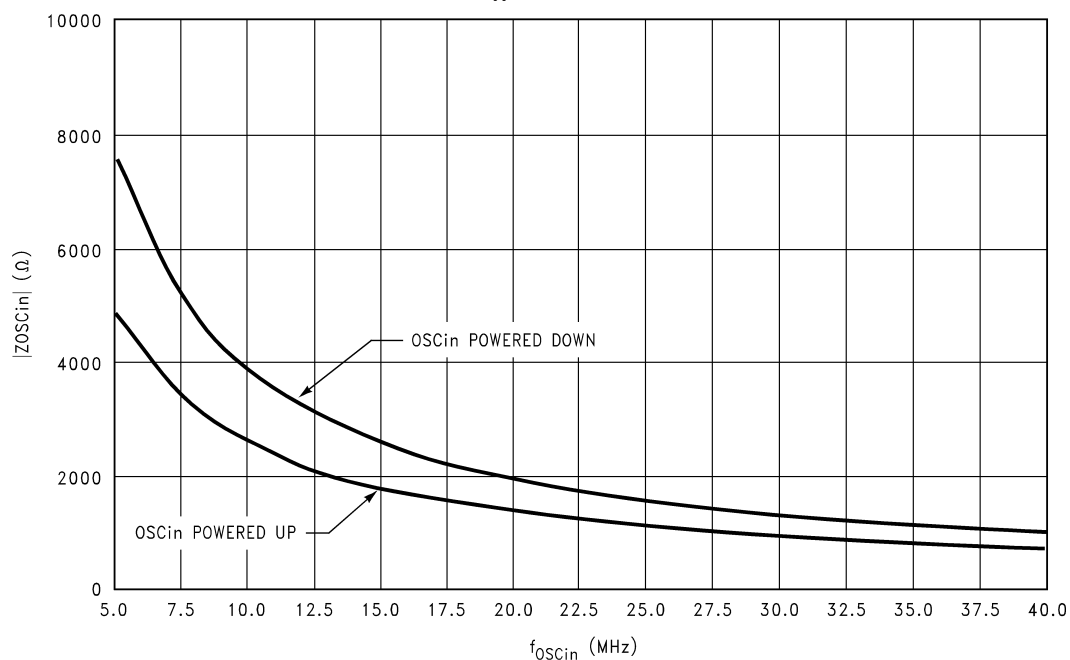
LMX233xU TSSOP OSCin Input Impedance Vs Frequency V_{CC} = EN = 2.50V T_A = +25^\circ C
