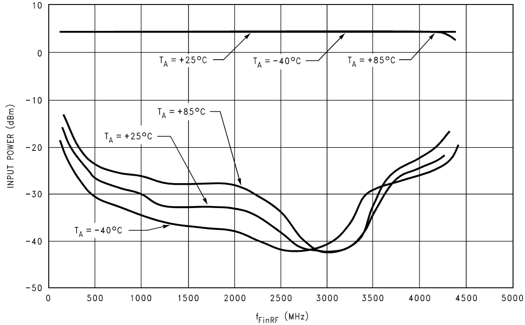
LMX2430 FinRF Input Power Vs Frequency Vcc = EN = 2.25V
