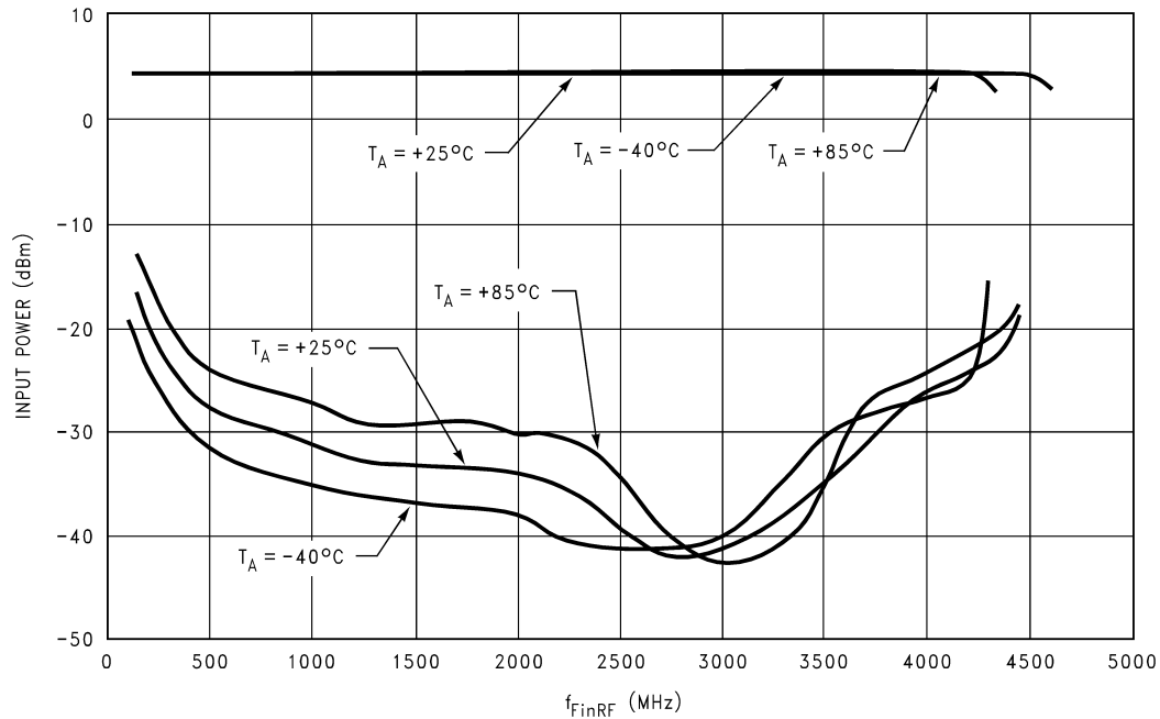
LMX2430 FinRF Input Power Vs Frequency Vcc = EN = 2.75V
