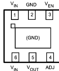
6-Lead LLP, Bottom View LP38693SD-ADJ
