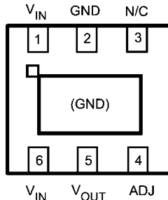
6-Lead LLP, Bottom View LP38691SD-ADJ
