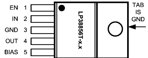
TO-220, Top View
