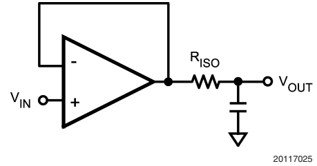
FIGURE 1. Resistive Isolation of Capacitive Load
