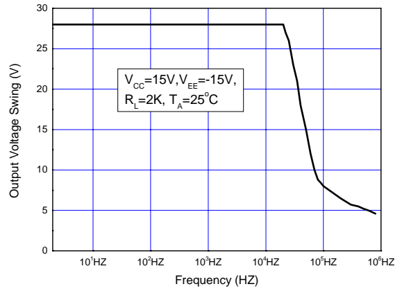
Figure 5. Maximum Output Voltage Swing vs. Frequency
