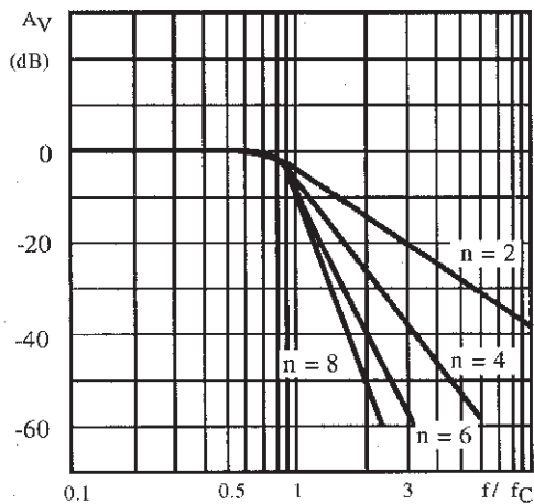
Figure 11 : Amplitude Response
