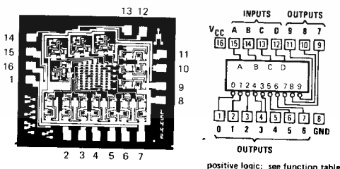
LS44 EXCESS-3-GRAY-TO-DECIMAL DECODER
