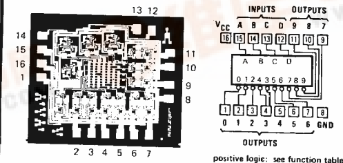
LS42 BCD-TO-DECIMAL DECODER
