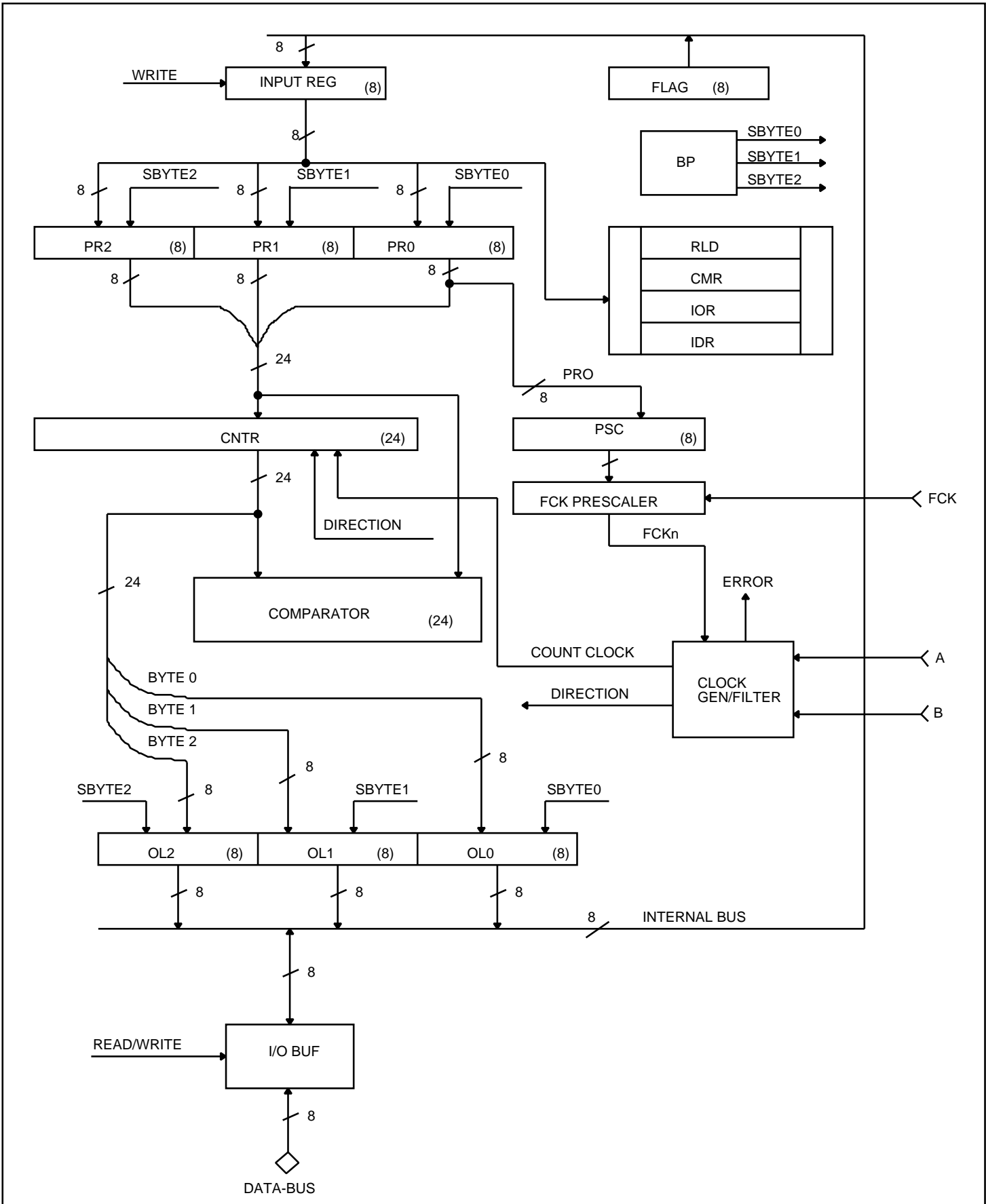
FIGURE 10. SINGLE-AXIS BLOCK DIAGRAM SHOWING MAJOR DATA PATHS
