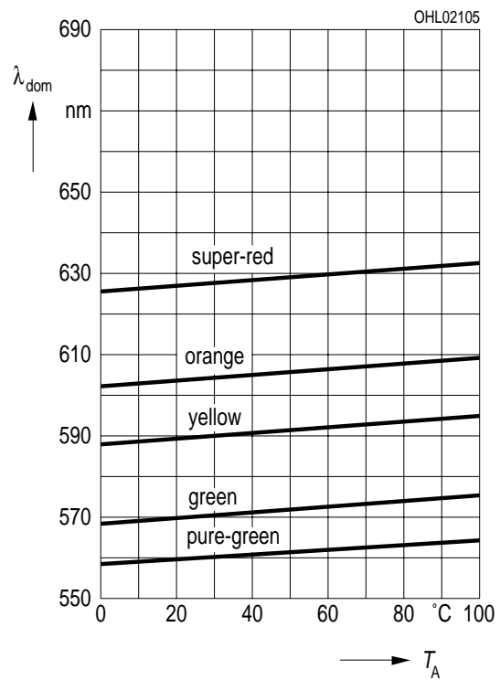
Dominantwellenlänge \lambda_{\text{dom}} = f(T_A) Dominant wavelength I_F = 10 \text{ mA}
