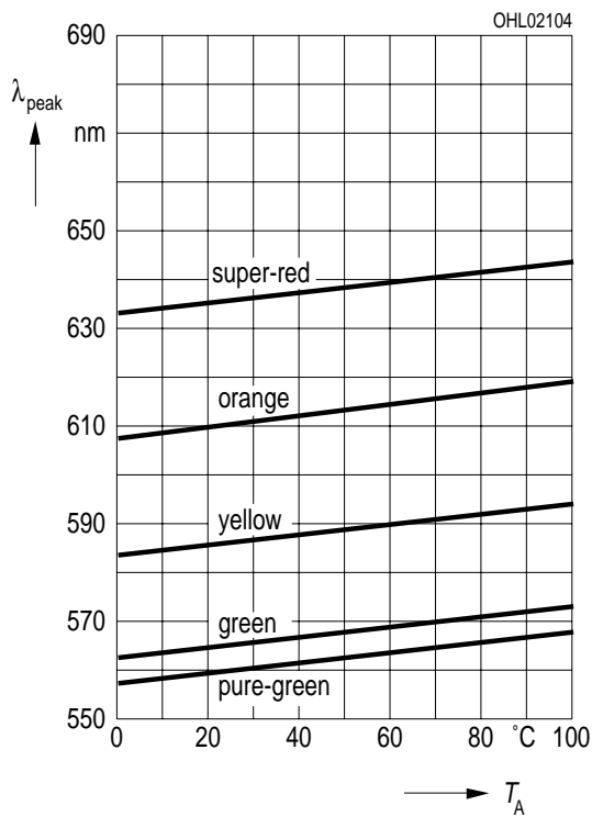
Wellenlänge der Strahlung \lambda_{\text{peak}} = f(T_A) Wavelength at peak emission I_F = 10 \text{ mA}
