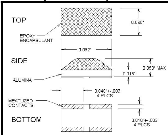
Figure 6 Outline Style 252A
