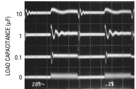
5V Transient Responses
