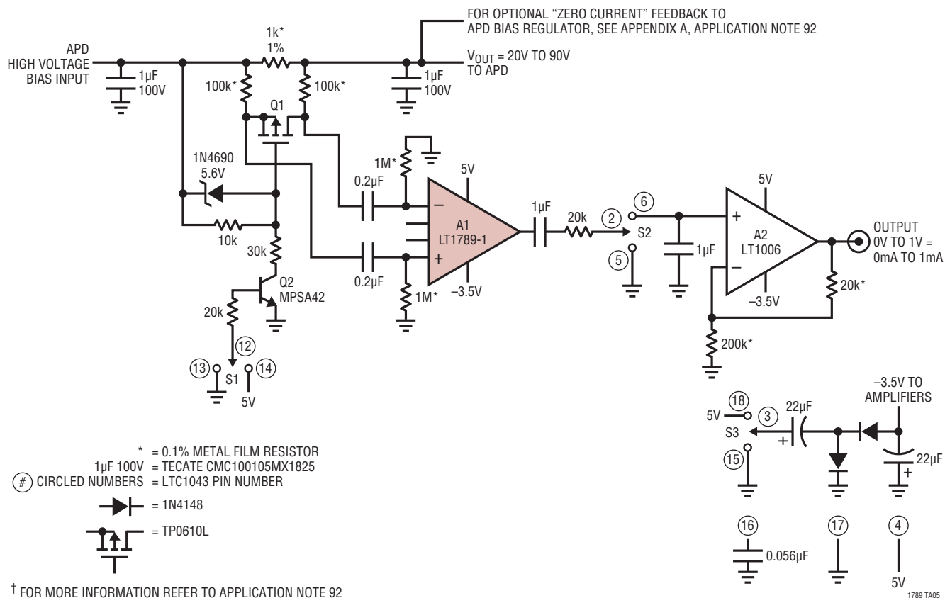
Avalanche Photo Diode Module Bias Current Monitor
