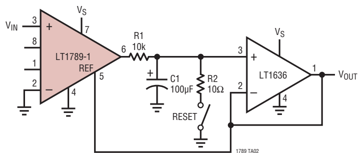
Single Supply Positive Integrator
