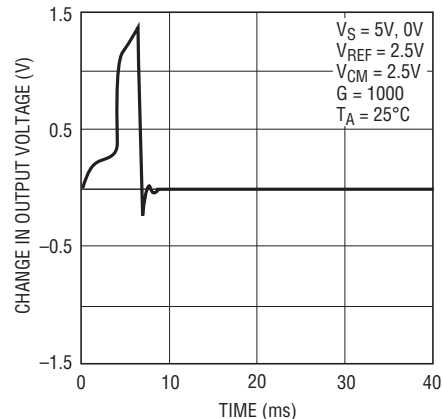
Turn-On Characteristics
