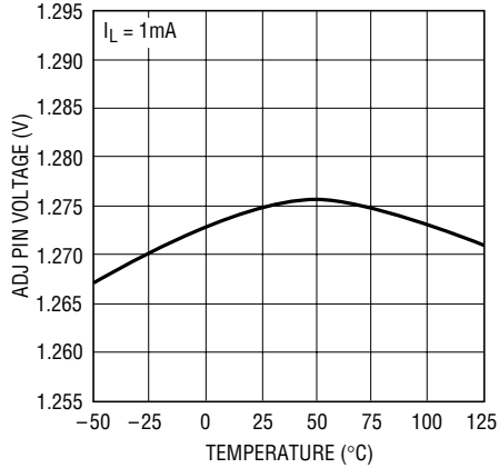
LT3010 ADJ Pin Voltage
