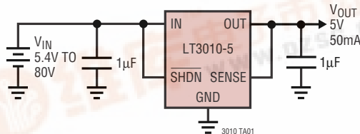
5V Supply with Shutdown
