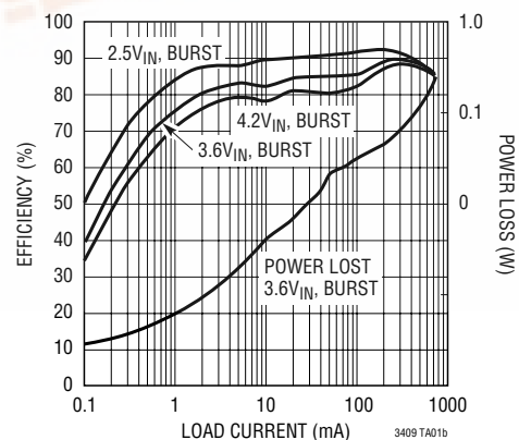
Burst Mode Efficiency, 1.8V OUT
