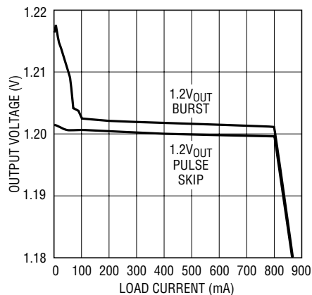
Output Voltage vs Load Current V_{IN} = 1.6V
