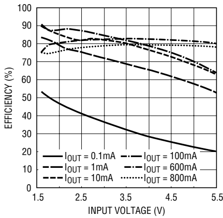
Efficiency vs Input Voltage V_{OUT} = 1.2V , Burst Mode Operation
