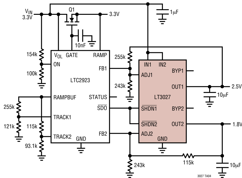
Power Supply Controller Provides Coincident Tracking
