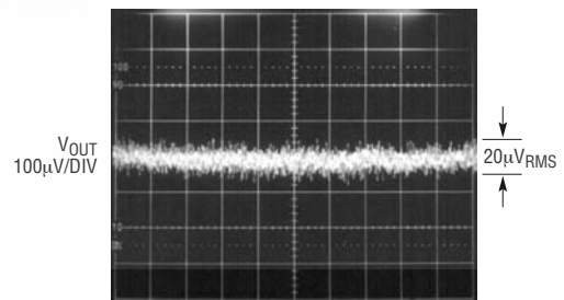
10Hz to 100kHz Output Noise
