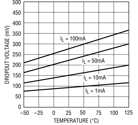
Dropout Voltage
