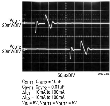
Channel-to-Channel Isolation
