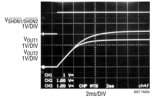
Noise Bypassing Slows Startup, Allows Outputs to Track
