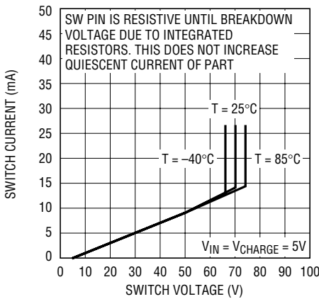
LT3468/LT3468-1 Switch Breakdown Voltage
