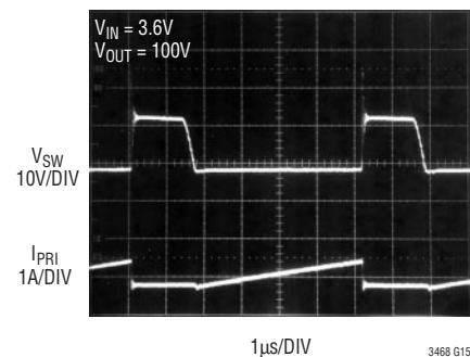
LT3468-1 Switching Waveform
