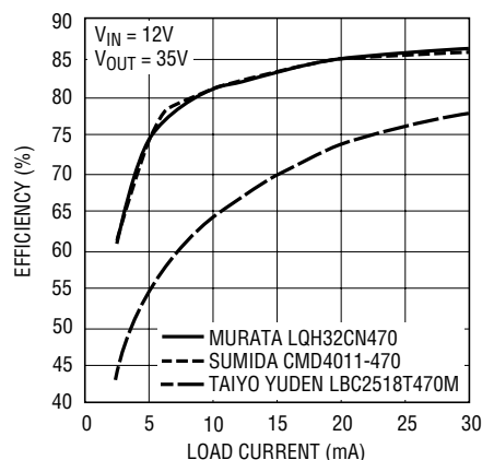
Figure 5. Efficiency Comparison of Different Inductors
