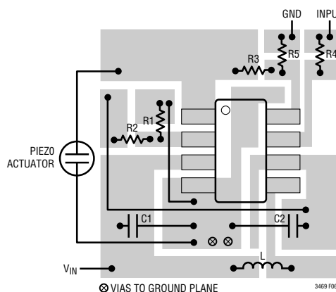
Figure 6. Recommended Component Placement
