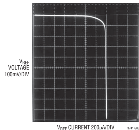
V REF Voltage vs V REF Current
