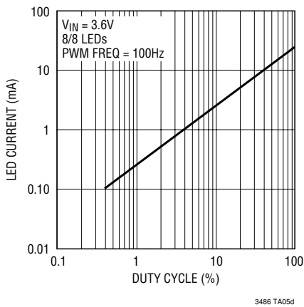
Wide (250:1) Dimming Range (LED Current 0.1mA to 25mA)
