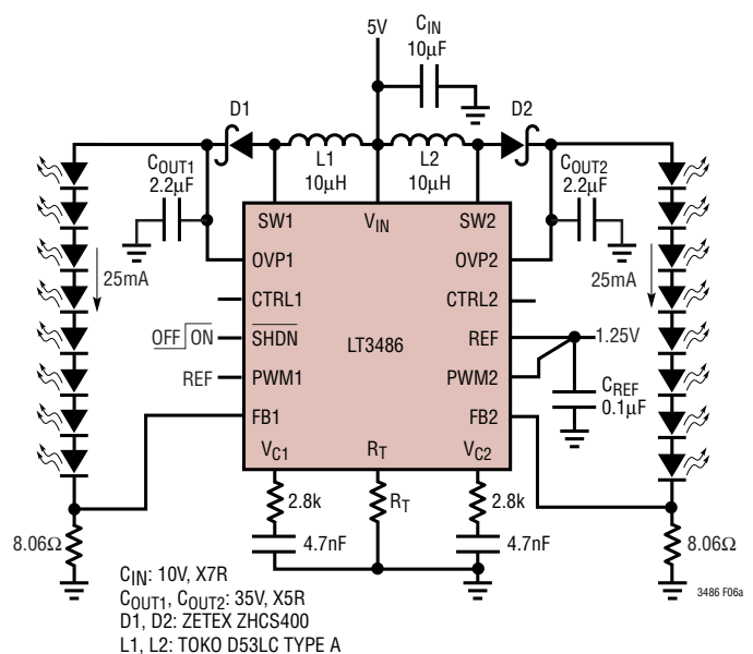
Figure 6a. 5V to 8/8 White LEDs
