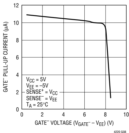
GATE - Pull-Up Current vs GATE - Voltage
