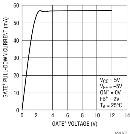
GATE + Pull-Down Current vs GATE + Voltage
